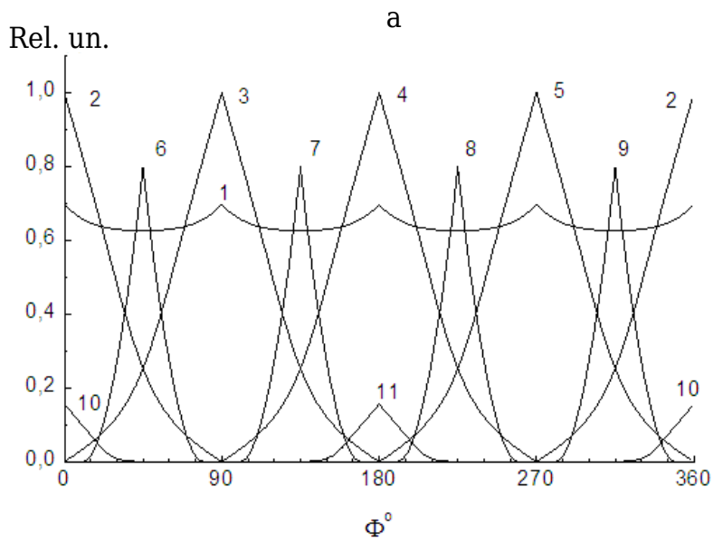
The azimuthal (a) and zenithal (b) directional diagrams of scintillation muon telescopes of the Yakutsk spectrograph at the surface of the Earth. The numbers correspond to the directions: for (a); 1- 0^\circ , 2 - N50^\circ , 3 - E50^\circ , 4 - S50^\circ , 5 - W50^\circ , 6 - NE60^\circ , 7 - ES60^\circ , 8 - SW60^\circ , 9 - WN60^\circ , 10 - N67^\circ , 11 - S67^\circ , for (b); 1- 0^\circ , 2 - 50^\circ , 3 - 60^\circ , 4 - 67^\circ
