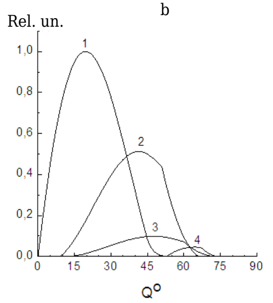
The azimuthal (a) and zenithal (b) directional diagrams of scintillation muon telescopes of the Yakutsk spectrograph at the surface of the Earth. The numbers correspond to the directions: for (a); 1- 0^\circ , 2 - N50^\circ , 3 - E50^\circ , 4 - S50^\circ , 5 - W50^\circ , 6 - NE60^\circ , 7 - ES60^\circ , 8 - SW60^\circ , 9 - WN60^\circ , 10 - N67^\circ , 11 - S67^\circ , for (b); 1- 0^\circ , 2 - 50^\circ , 3 - 60^\circ , 4 - 67^\circ
